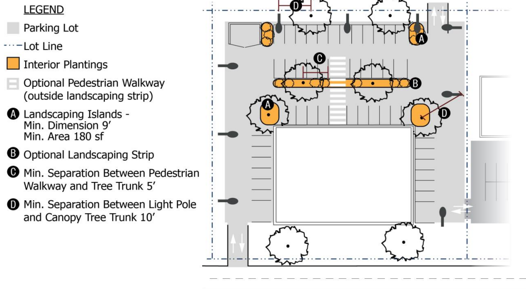
FIGURE 6.6.11.A: PARKING LOT INTERIOR PLANTINGS
