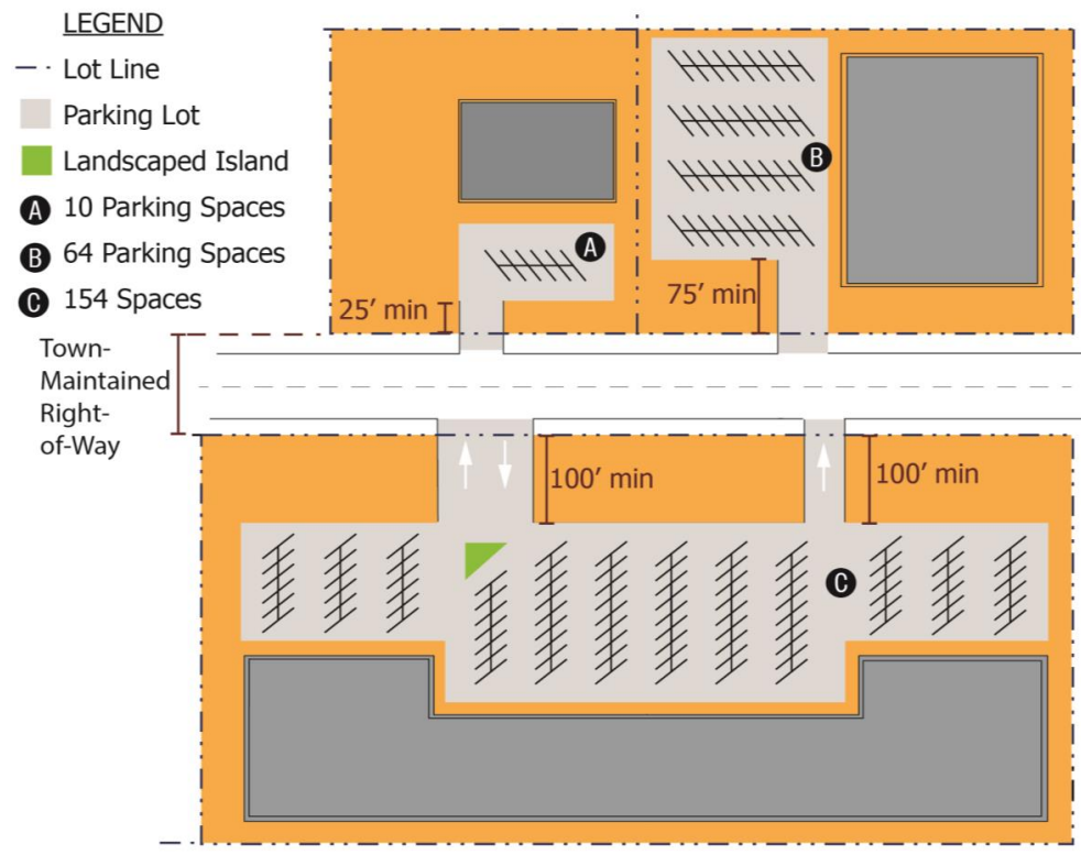
FIGURE 6.1.4.E: PARKING LOT ACCESSWAY DEPTH
