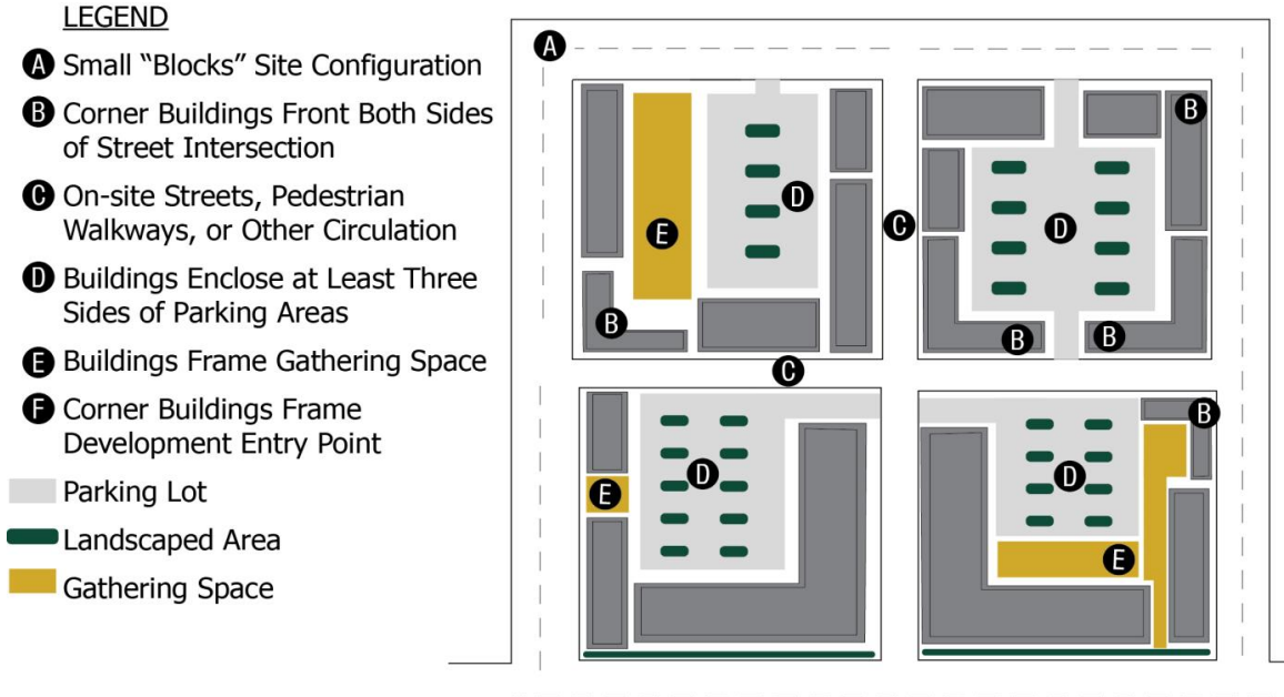
FIGURE 6.2.3.E.2: MULTI-BUILDING DEVELOPMENT
