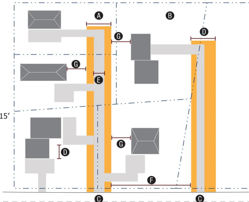
FIGURE 6.1.4.D.5: ALTERNATIVE LOT ACCESS
